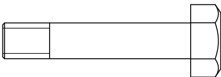
M10*50 6PCS
